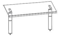
47" HIGH BREATH GUARD H24.5" | gap H14" H62cm | gap H36.5cm Fits medium units MG CIAN04 X _ XX
