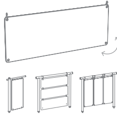
LONG BLACKBOARD L47" H18" L120cm H45cm Fits Arch and Sign post MG SADDSM 02
