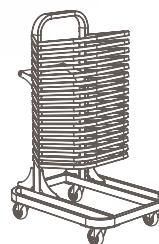
ROUND / SQUARE TOP TRANSFER AND STORAGE CART L40" W31" H61" L101cm W79cm H155cm holds up to 16 CliX round/square tops
